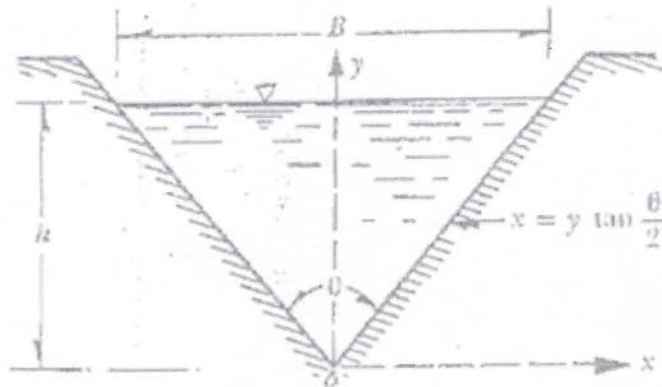
Figura 3 Vertedero Triangular
