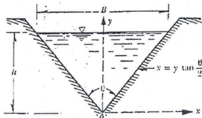
Figura 3 Vertedero Triangular
